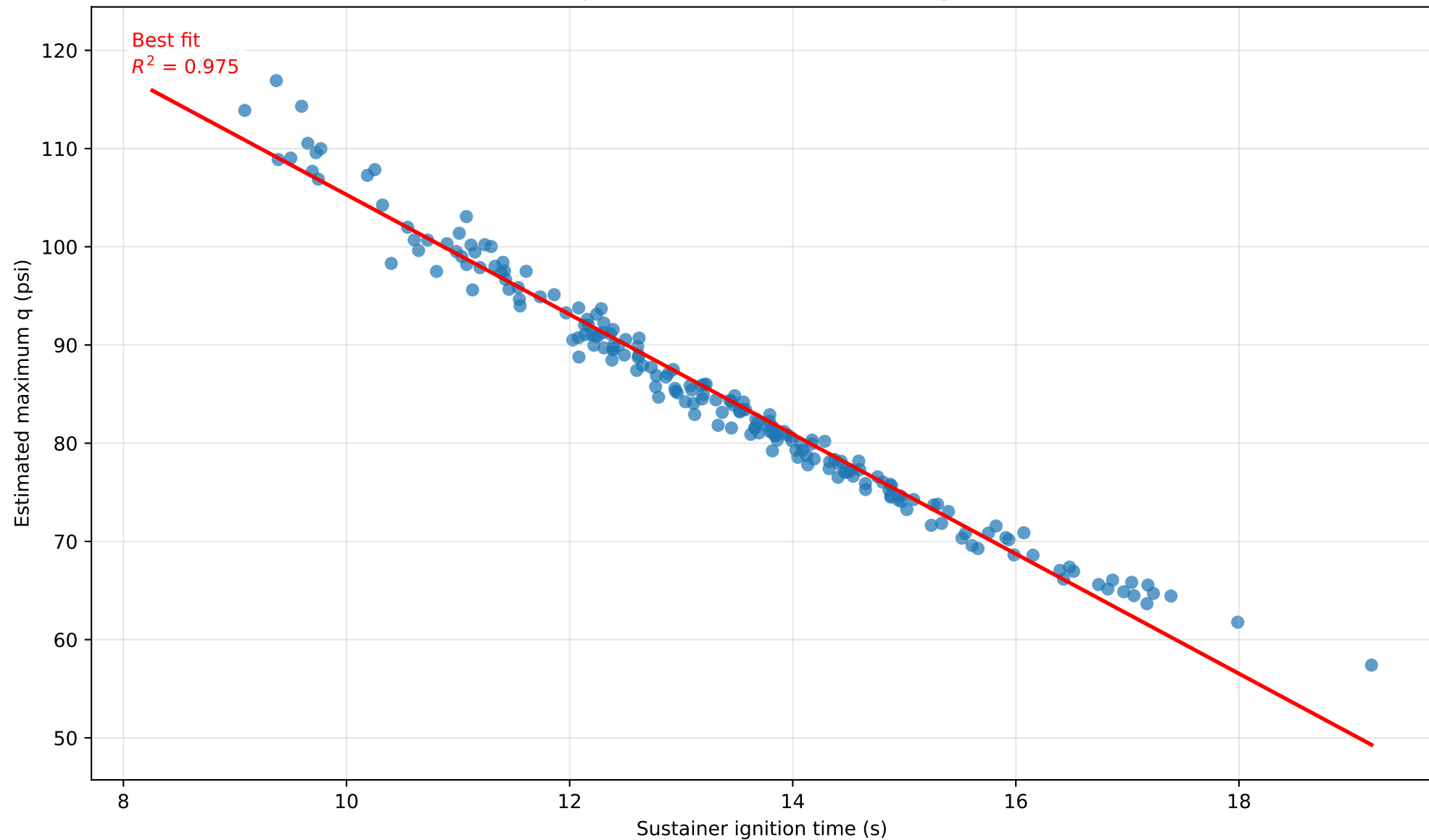
Maximum Dynamic Pressure vs Sustainer Ignition Time
